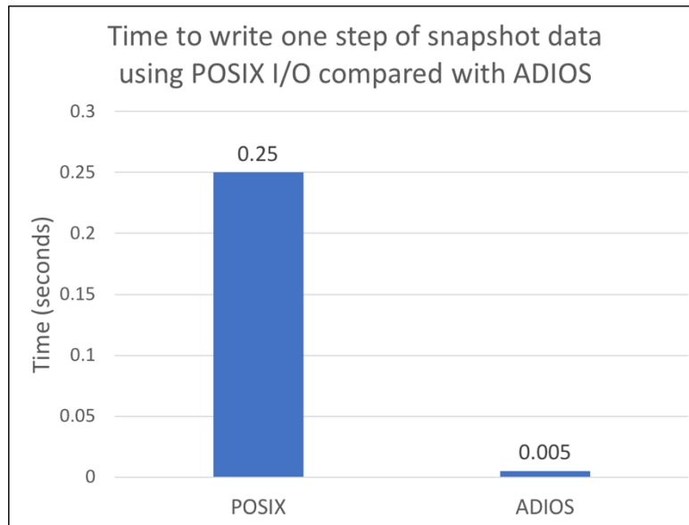
Figure 1: Comparison of the time taken to write one snapshot of GTC on Summit to the GPFS parallel file system for POSIX vs. ADIOS
