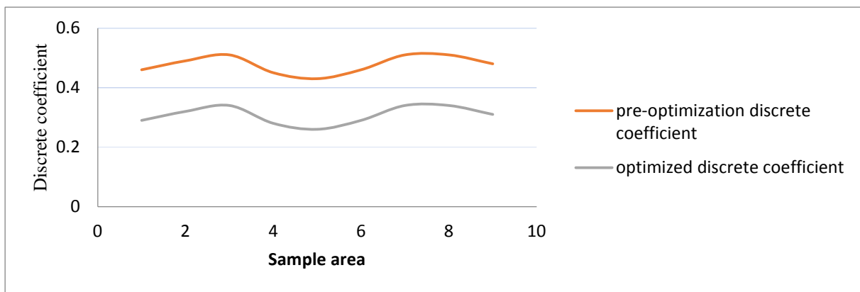
Figure 14. CV curve before and after optimization in different regions
