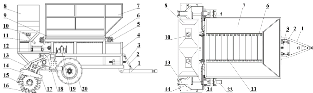
Figure 1. Main view of the machine Figure 2. Vertical view of the machine
