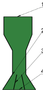
1 Fertilizer-in port 2 Fertilizer-transfer port 3 Fertilizer plug-in plate 4 Fertilizer-out port
