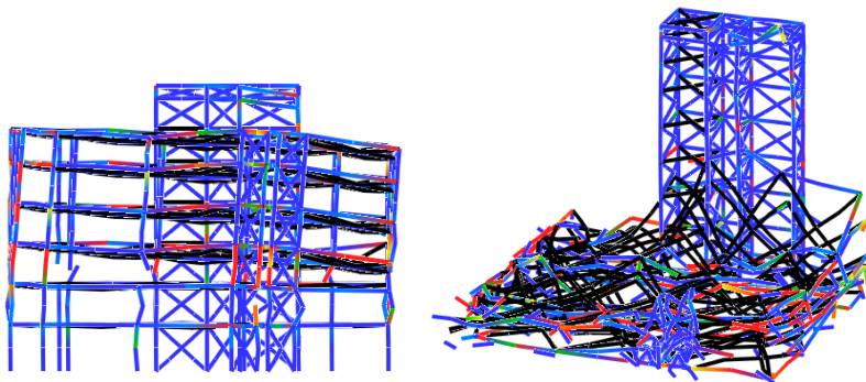
Fig.1 Collapse analysis of the CTV building
