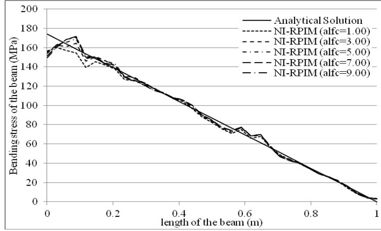
Figure 10. Comparison of effect of \text{alfc} (\alpha_c) on bending stress results of cantilever beam for nodal int. with ASD ( 0^{\text{th}} order term).
