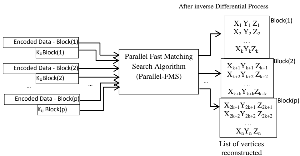
(a) Vertices (X,Y and Z) reconstructed
